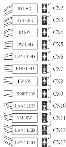
LED Connector
