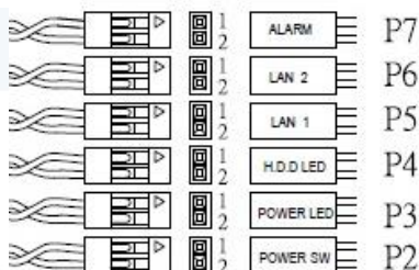
LED Connector
