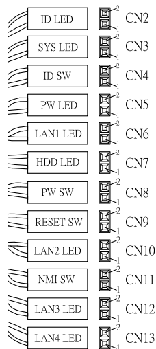
LED Connector
