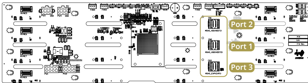
Host Side
